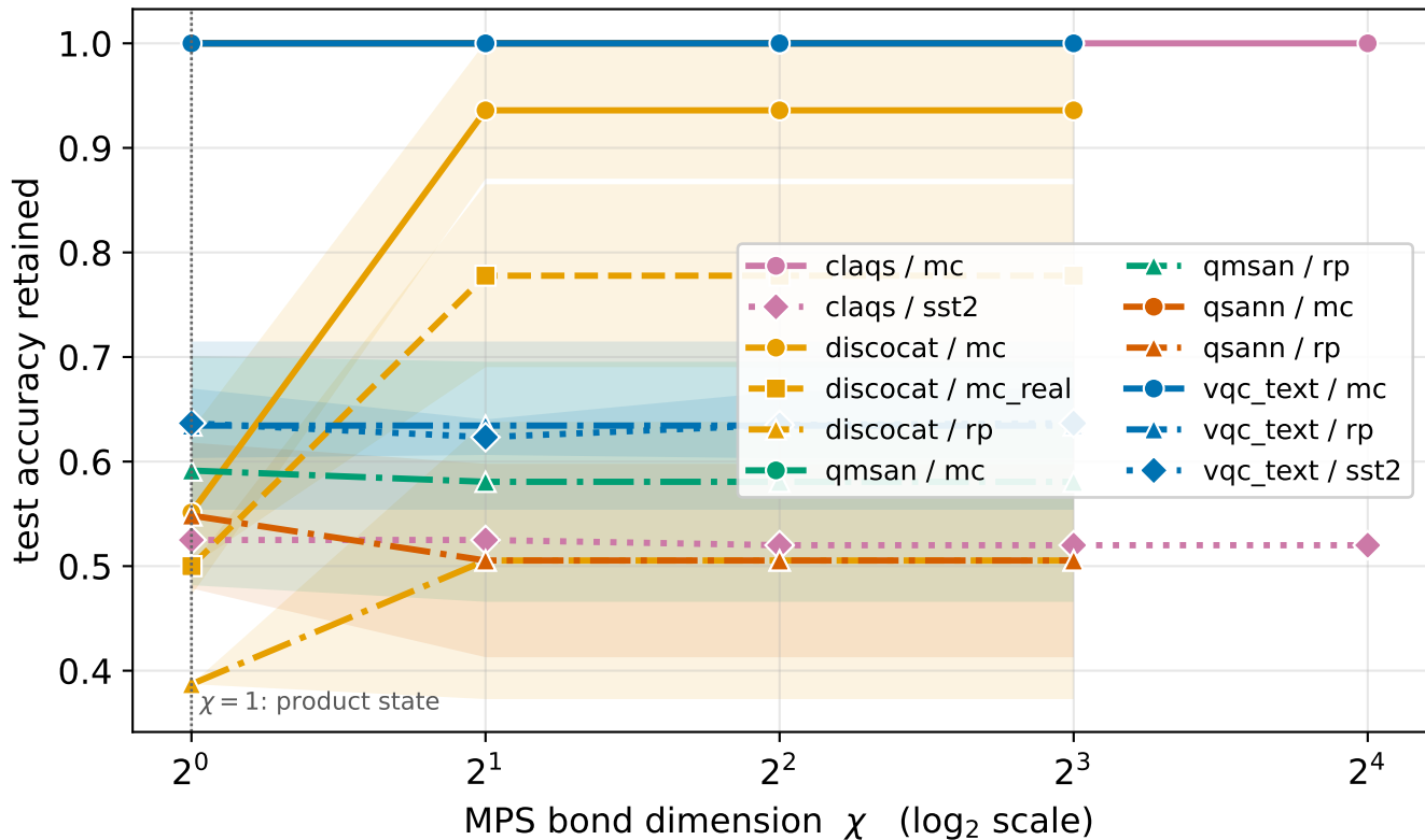
A classical surrogate recovers the predictions at small \chi
