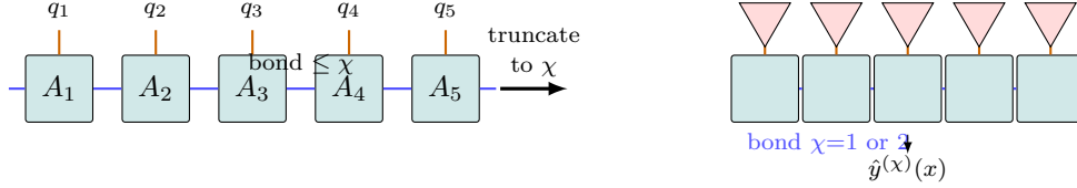
Figure 4: The audit in tensor-network terms. Any trained variational model is a matrix product state (MPS) whose bond dimension caps the entanglement it carries [Shin et al., 2024]. SIMCERT truncates that MPS to bond dimension \chi (right; blue bond legs, orange physical legs q_i , red readout observables) and asks how small \chi can be before the recovered prediction \hat{y}^{(\chi)} changes. For every audited model the answer is \chi=1 (a product state) or \chi=2 , while an exact representation would need bond dimension 2^{\lfloor n/2 \rfloor} .
