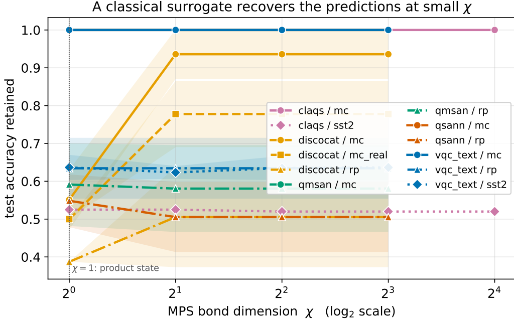
Figure 6: Accuracy retained versus bond dimension , one curve per model and dataset, mean and standard deviation over seeds. Color encodes the model and the line style and marker encode the dataset, so each series is distinguishable by shape as well as color. Flat curves down to \chi=1 are the signature of a bond-cheap model, since the classical surrogate loses nothing as it is weakened. The SST-2 series sit lower, being a real and non-separable task, but are equally flat in \chi .
