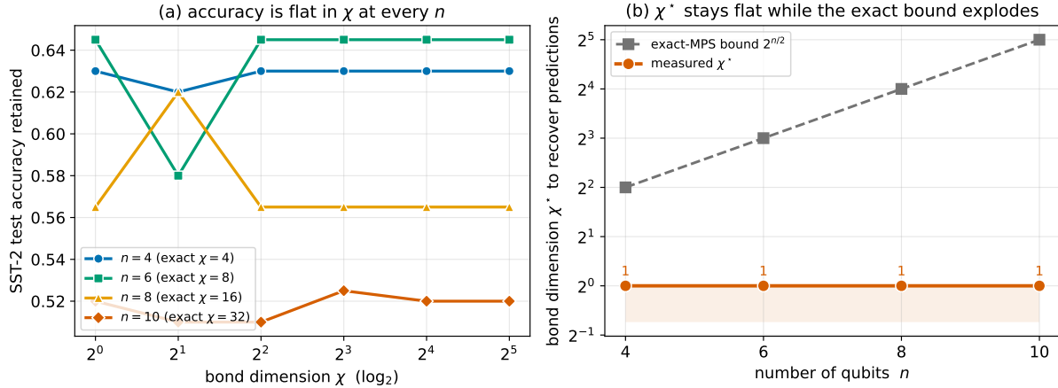
Figure 5: \chi^* does not grow with qubit count . Left, accuracy retained versus bond dimension for the reference model at n \in \{4, 6, 8, 10\} on SST-2; each curve is flat down to \chi=1 . Right, the measured \chi^* (orange) stays at 1 while the exact-MPS bound 2^{n/2} (grey, dashed) grows exponentially on the log axis. A product-state surrogate recovers the predictions at every size tested. Accuracy here is modest and does not rise with n , so this probes recovery rather than a strong classifier.
