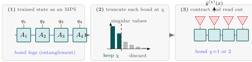
Figure 4: The audit in tensor-network terms. Any trained variational model is a matrix product state whose bond dimension caps the entanglement it carries (Shin et al., 2024). (1) We write the trained state |\psi_\theta(x)\rangle as an MPS, with orange physical legs q_i and blue bond legs. (2) For each bond we keep only the largest \chi singular values and discard the rest, the standard MPS truncation. (3) SIMCERT contracts the \chi -capped MPS with the red readout observables and asks how small \chi can be before the recovered prediction \hat{y}^{(\chi)} changes. For every audited model the answer is \chi=1 , a product state, or \chi=2 , whereas an exact representation would need bond dimension 2^{\lfloor n/2 \rfloor} .
