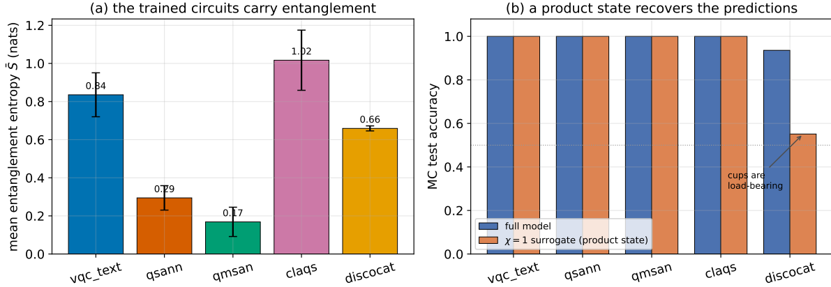
Figure 7: Entanglement is present but, with one exception, not load-bearing (MC, all five models). Left, the mean bipartite entanglement entropy \bar{S} is non-zero for every model, so the trained states are genuinely entangled. Right, the full model and its \chi=1 product-state surrogate reach the same accuracy for the attention and mixer models, whereas for discocat the \chi=1 surrogate drops toward chance, marking the one place where the entanglement built by its grammar cups is load-bearing.
