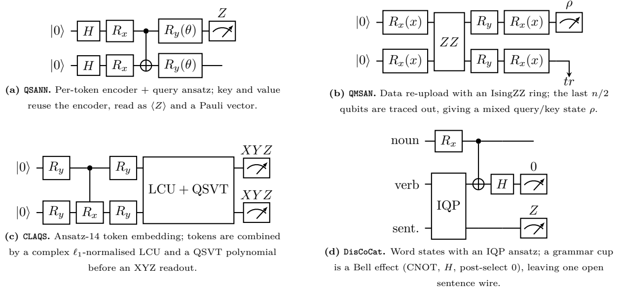
Figure 9: Representative circuits for the audited models (simplified; exact per-model circuits are released with the harness). QMSAN is read out as a reduced density matrix, which is why it uses the mixed-state audit path; DisCoCat post-selects the cup qubits and reads the single open wire by the Born rule.
