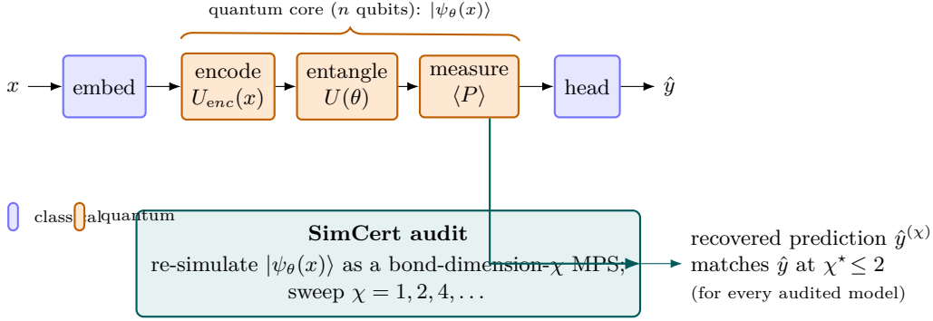
Figure 1: What the audit interrogates. A trained QNLP classifier (top) threads a sentence x through a classical embedding (blue), a quantum core (orange: encode, entangle, measure) that prepares |\psi_\theta(x)\rangle , and a classical head, producing a label \hat{y} . SIMCERT (bottom, teal) replaces the quantum core with a classical matrix-product-state surrogate of bond dimension \chi and sweeps \chi to find the smallest value that still recovers the model’s own predictions. For every audited model that value is 1 or 2.
