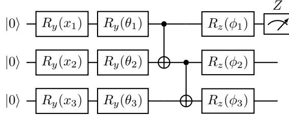
Figure 3: Representative variational ansatz (the reference classifier; the attention and mixer models use the same primitives). Each input feature is angle-encoded ( R_y(x_i) ), followed by a trainable layer ( R_y(\theta_i) ), a CNOT entangling chain, and a trainable R_z(\phi_i) . The block repeats L times with the data re-uploaded each layer, and the class is read from \langle Z_0 \rangle . The audit forms the bond-dimension- \chi MPS approximation of the state prepared just before measurement. Per-model circuits (including qmsan ’s mixed-state readout and claqs ’s LCU/QSVT block) are in Appendix B.
