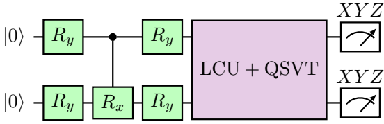
(c) CLAQS . Ansatz-14 token embedding; tokens are combined by a complex \ell_1 -normalised LCU and a QSVT polynomial before an XYZ readout.
