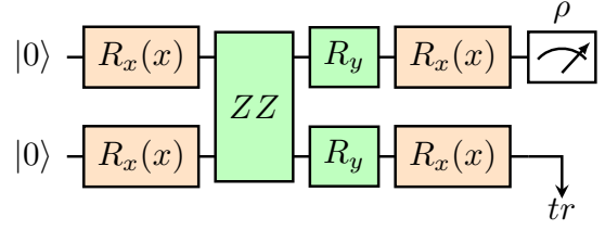
(b) QMSAN . Data re-upload with an IsingZZ ring; the last n/2 qubits are traced out, giving a mixed query/key state \rho .
