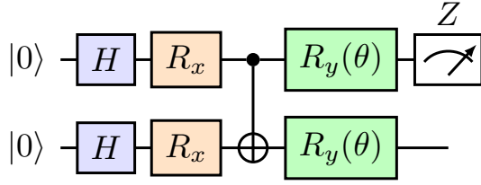
(a) QSAN . Per-token encoder plus a query ansatz; key and value reuse the encoder, read as \langle Z \rangle and a Pauli vector.
