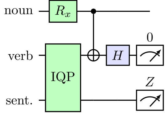
(d) DisCoCat . Word states with an IQP ansatz; a grammar cup is a Bell effect (CNOT, H , post-select 0), leaving one open sentence wire.
