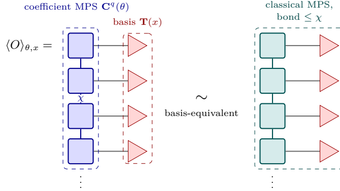
Figure 4: Following the dequantization picture of Shin et al. (2024), the trained model’s expectation value is a coefficient matrix product state \mathbf{C}^q(\theta) (blue) contracted with a fixed set of basis functions \mathbf{T}(x) (red), and its bond dimension caps the entanglement it can carry. If that bond dimension is small, a classical MPS of the same size (teal) contracts with the same basis functions to reproduce the output, so the model is basis-equivalent to a cheap classical one. SIMCERT measures this bond dimension directly: it truncates the trained state to bond dimension \chi and finds the smallest \chi that still recovers the predictions, which for every audited model is 1 or 2, against an exact-representation bound of 2^{\lfloor n/2 \rfloor} .
