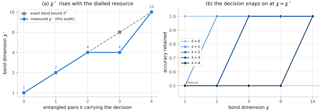
Figure 7: The audit discriminates. Left, measured \chi^* against the number of entangled pairs k carrying the decision, with the exact bond bound 2^k dashed; the two coincide except at k=3 . Right, retained accuracy against \chi for each k : the decision sits at chance until \chi reaches \chi^* , then snaps to 1.0. Qubit count, wire order, readout and readout weight are identical at every k , so the only thing varying along these curves is the entanglement the decision depends on.
