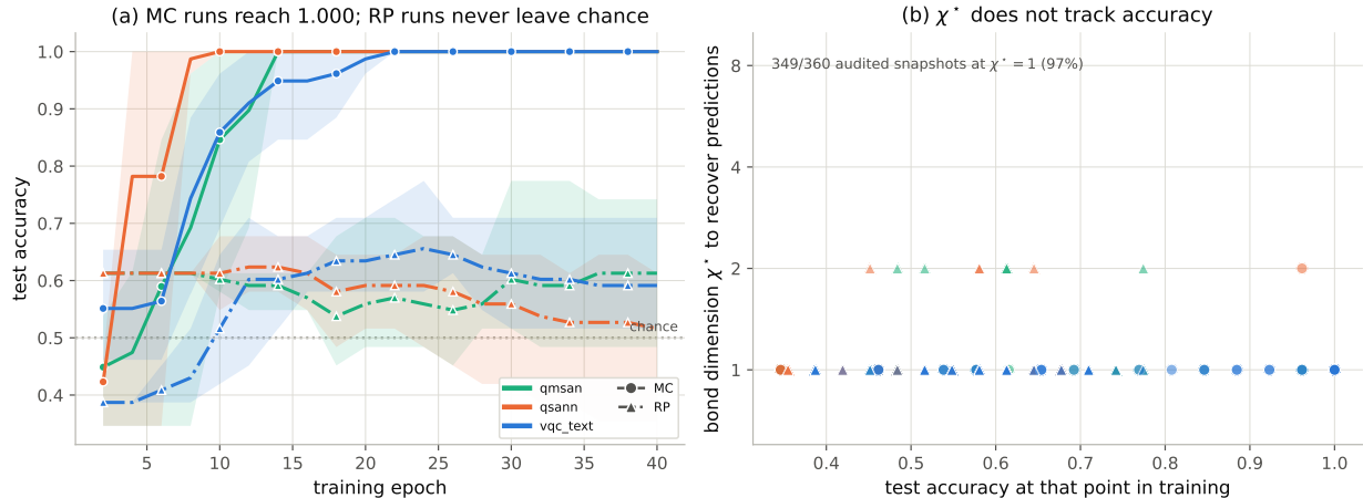
Figure 8: The verdict does not depend on the model having failed to learn. Left, test accuracy against training epoch, mean over three seeds with the seed range shaded; mc runs (solid, circles) go from chance to 1.000, while rp runs (dash-dot, triangles) never leave chance. Right, \chi^* at every one of those snapshots against the accuracy reached there. If the audit were merely detecting undertrained models, \chi^* would rise to the right; it does not, and every snapshot at accuracy 1.000 certifies \chi^*=1 .
