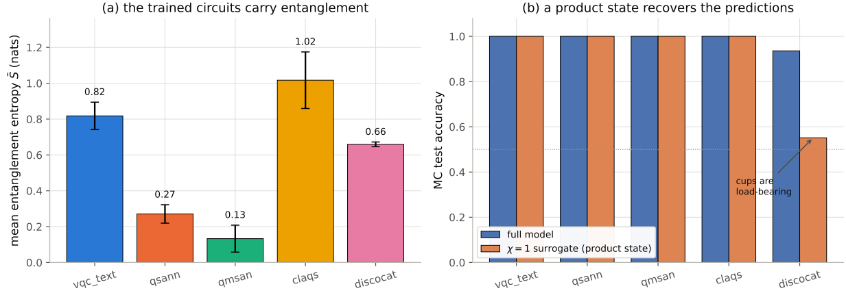
Figure 11: Entanglement is present but, with one exception, not load-bearing, on MC for all five models). Left, the mean bipartite entanglement entropy \bar{S} is non-zero for every model, so the trained states are genuinely entangled. Right, the full model and its \chi=1 product-state surrogate reach the same accuracy for the attention and mixer models, whereas for discocat the \chi=1 surrogate drops toward chance, marking the one place where the entanglement built by its grammar cups is load-bearing.
