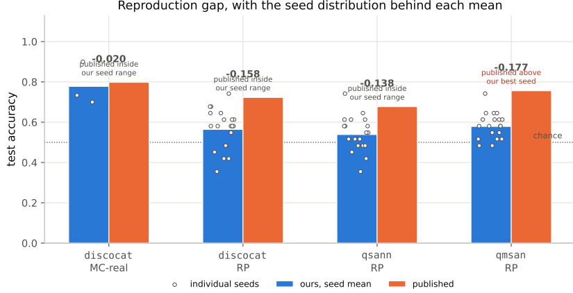
Figure 10: Reproduction gap, with the seed distribution behind each mean. Bars are our seed mean against the published number; the bold annotation is ours minus published, and each open circle is one seed. MC-REAL reproduces to within 0.02. On RP, a fragile task of only 74 training items reimplemented with our own embeddings and an offline reader, the mean runs below published, but the seed spread is wide enough that the published value falls inside our range for discocat and qsann , and 0.014 above our best seed for qmsan . Seed means and counts here are produced by the same selection rule as Table 3, so the figure and the table report the same quantity. The simulability verdict concerns our own trained circuits and does not depend on closing this gap.
