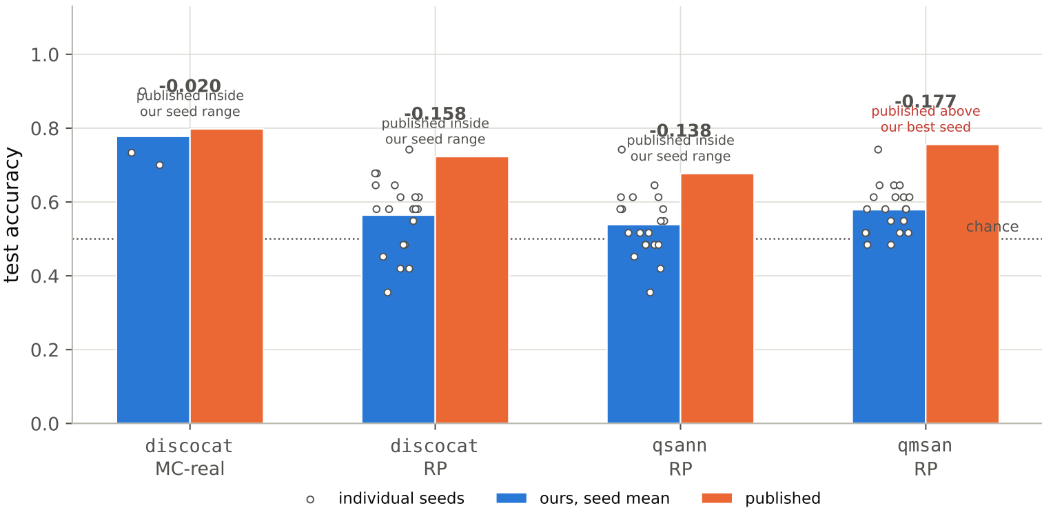
Reproduction gap, with the seed distribution behind each mean
