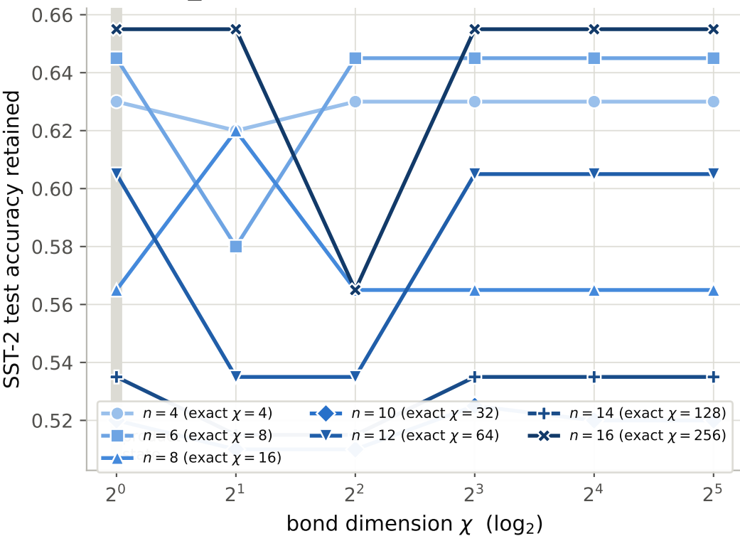
(a) \text{vqc\_text} : \chi = 1 matches the full model at every n
