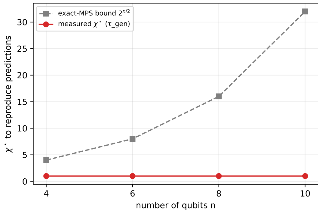
(b) Required bond dimension vs n
