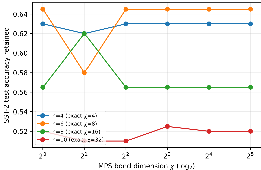
(a) Accuracy vs \chi , per qubit count
