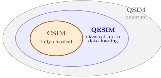
Figure 2: Which simulability we claim. The standard hierarchy: classically simulable (CSIM) \subseteq classically simulable up to a data-loading step (QESIM) \subseteq quantum-simulable (QSIM) (Cerezo et al., 2025; Shin et al., 2024). Our MPS surrogate realises CSIM when the required bond dimension is small, and we make no claim outside that regime.
