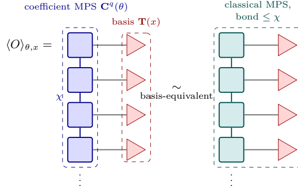
Figure 4: The audit in tensor-network terms (following the dequantization picture of Shin et al., 2024). The trained model’s expectation value is a coefficient matrix product state \mathbf{C}^q(\theta) (blue) contracted with a fixed set of basis functions \mathbf{T}(x) (red), and its bond dimension caps the entanglement it can carry. If that bond dimension is small, a classical MPS of the same size (teal) contracts with the same basis functions to reproduce the output, so the model is basis-equivalent to a cheap classical one. SIMCERT measures this bond dimension directly: it truncates the trained state to bond dimension \chi and finds the smallest \chi that still recovers the predictions, which for every audited model is 1 or 2, against an exact-representation bound of 2^{\lceil n/2 \rceil} .
