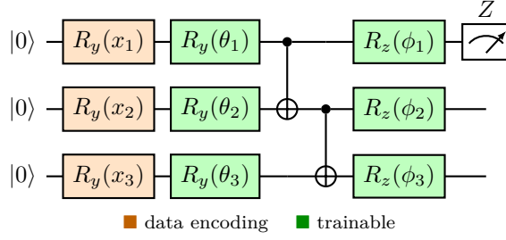
Figure 3: Representative variational ansatz (the reference classifier; the attention and mixer models use the same primitives). Each input feature is angle-encoded ( R_y(x_i) , orange), followed by a trainable layer ( R_y(\theta_i) , green), a CNOT entangling chain, and a trainable R_z(\phi_i) . The block repeats L times with the data re-uploaded each layer, and the class is read from \langle Z_0 \rangle . The audit forms the bond-dimension- \chi MPS approximation of the state prepared just before measurement. Per-model circuits are in Appendix B.
