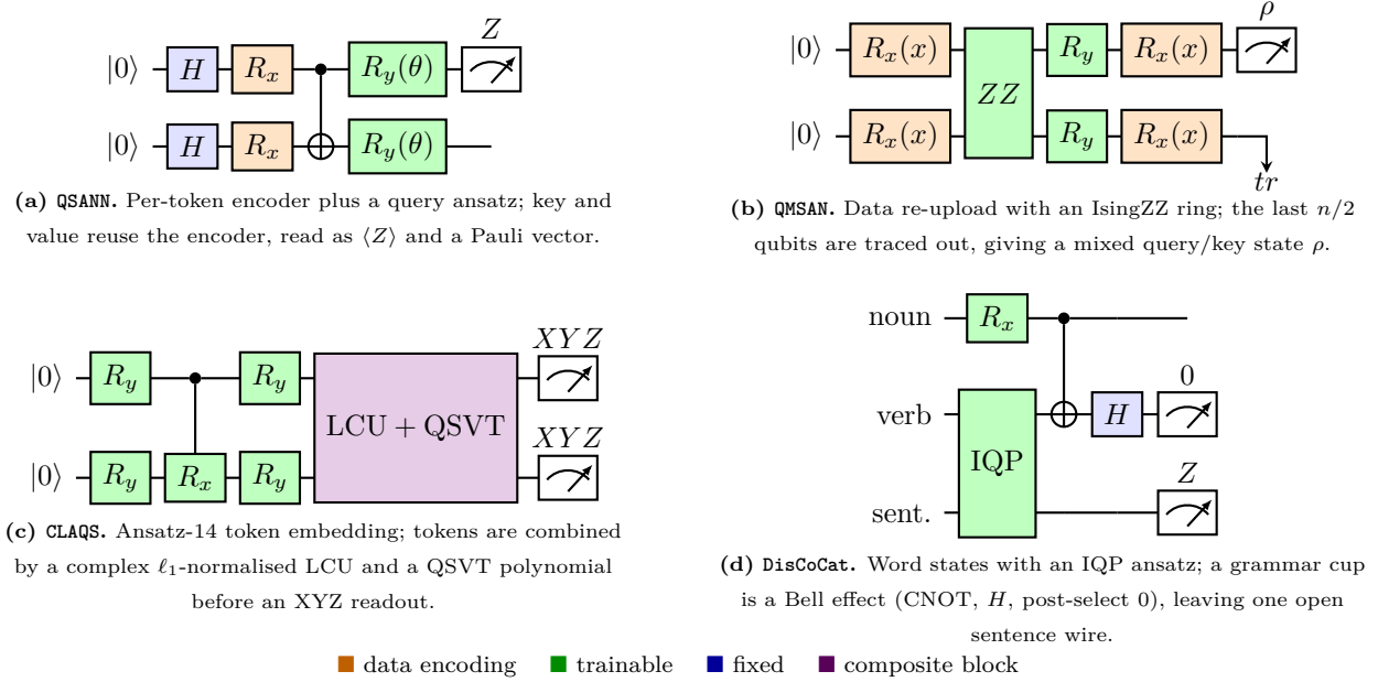
Figure 9: Representative circuits for the audited models (simplified; exact per-model circuits are released with the harness). Gates are colored by role. QMSAN is read out as a reduced density matrix, hence the mixed-state audit path; DisCoCat post-selects the cup qubits and reads the single open wire by the Born rule.
