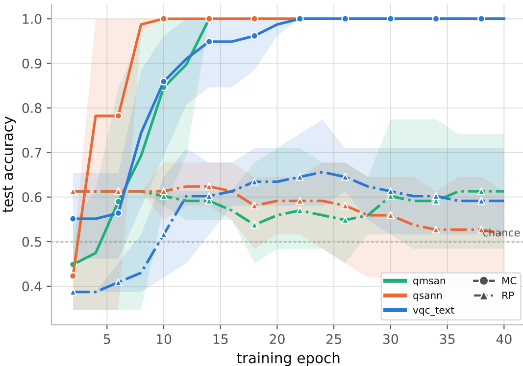
(a) MC runs reach 1.000; RP runs never leave chance
