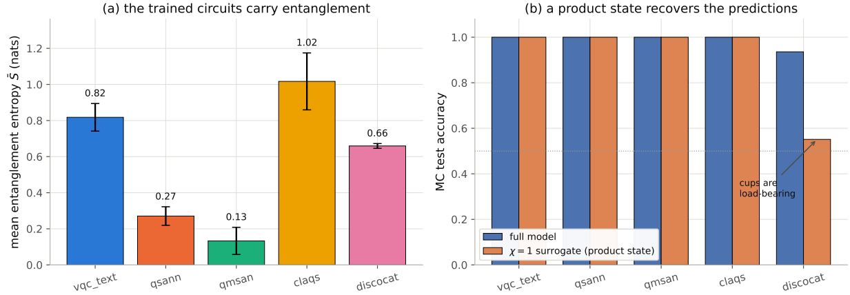
Figure 12: Entanglement is present but, with one exception, not load-bearing, on MC for all five models). Left, the mean bipartite entanglement entropy \tilde{S} is non-zero for every model, so the trained states are genuinely entangled. Right, the full model and its \chi=1 product-state surrogate reach the same accuracy for the attention and mixer models, whereas for discocat the \chi=1 surrogate drops toward chance, marking the one place where the entanglement built by its grammar cups is load-bearing.
