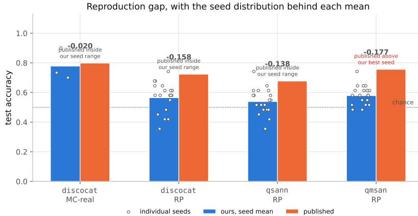
Figure 11: Reproduction gap, with the seed distribution behind each mean. Bars are our seed mean against the published number; the bold annotation is ours minus published, and each open circle is one seed. MC-REAL reproduces to within 0.02. On RP, a fragile task of only 74 training items reimplemented with our own embeddings and an offline reader, the mean runs below published, but the seed spread is wide enough that the published value falls inside our range for discocat and qsann , and 0.014 above our best seed for qmsan . Seed means and counts here are produced by the same selection rule as Table 3, so the figure and the table report the same quantity. The simulability verdict concerns our own trained circuits and does not depend on closing this gap.
