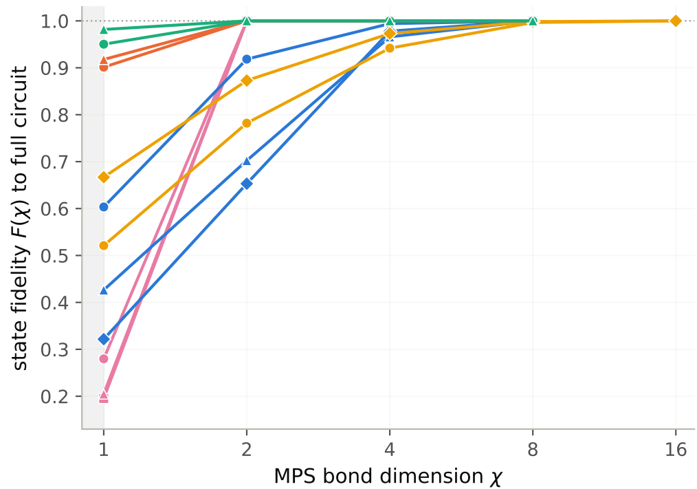
(b) state fidelity climbs with \chi
