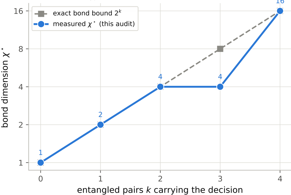
(a) \chi^* rises with the dialled resource
