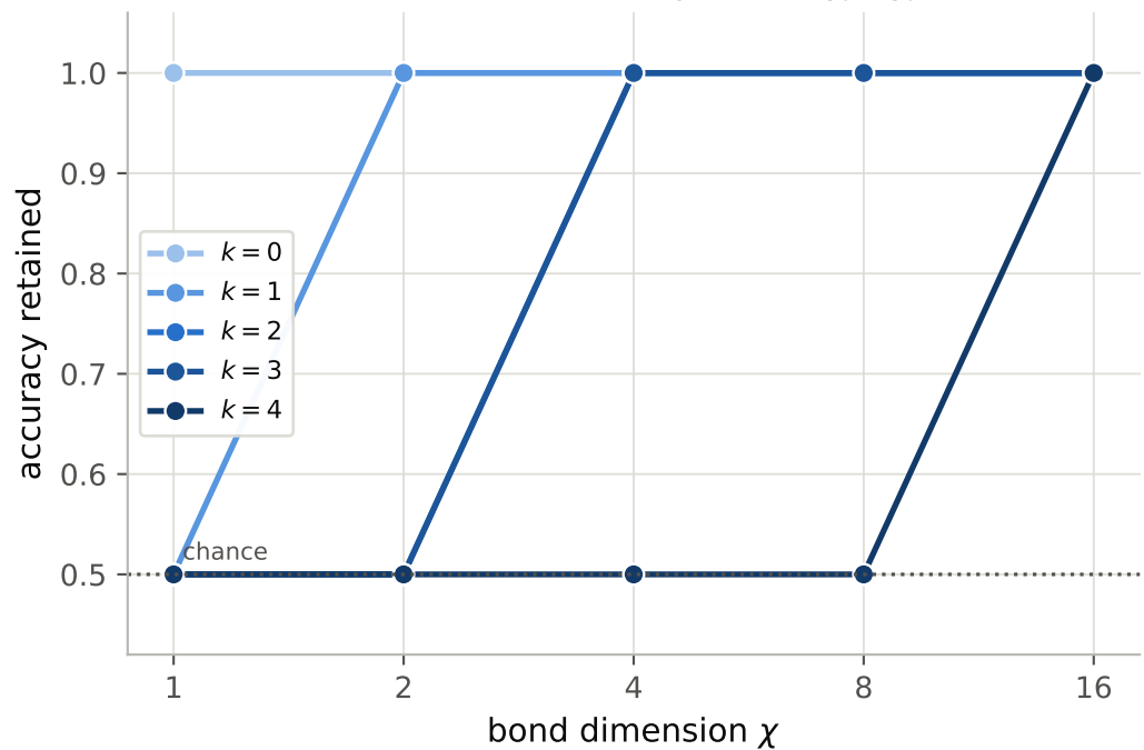
(b) the decision snaps on at \chi = \chi^*
