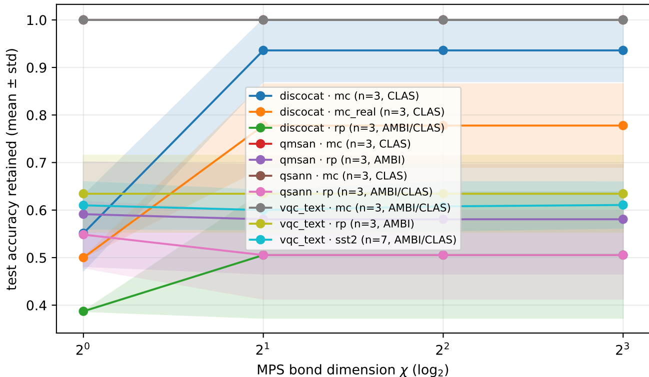
Was the quantum load-bearing? Accuracy retained vs bond dimension
