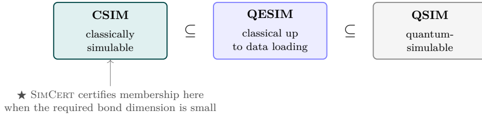
Figure 2: The nested hierarchy of classical simulability. A classically simulable model (CSIM) is a special case of one that is simulable up to a data-loading step (QESIM), which is a special case of quantum-simulable (QSIM) (Cerezo et al., 2025; Shin et al., 2024). SIMCERT certifies membership in CSIM whenever the trained state truncates to a small bond dimension, and we make no claim outside that innermost class.
