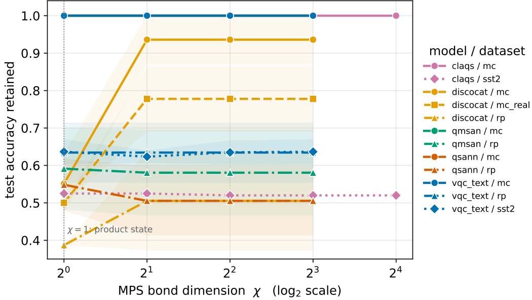
Figure 6: Accuracy retained versus bond dimension, one curve per model and dataset, mean and standard deviation over seeds. Color encodes the model and the line style and marker encode the dataset, so each series is distinguishable by shape as well as color. Flat curves down to \chi=1 are the signature of a bond-cheap model, since the classical surrogate loses nothing as it is weakened. The SST-2 series sit lower, being a real and non-separable task, but are equally flat in \chi .
