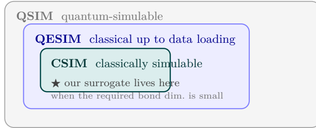
Figure 2: The nested hierarchy of classical simulability. A model that is classically simulable (CSIM) is a special case of one that is simulable up to a data-loading step (QESIM), which in turn is a special case of quantum-simulable (QSIM) (Cerezo et al., 2025; Shin et al., 2024). Our matrix-product-state surrogate certifies membership in CSIM whenever the required bond dimension is small, and we make no claim outside that innermost region.
