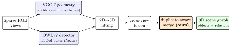
Fig. 1. Architecture of the detector-grounded sparse-view 3D scene graph system. Sparse RGB frames pass through frozen VGGT (camera/depth/world-point/confidence maps) and a frozen open-vocabulary detector (OWLv2), which proposes labeled object boxes. Each detection is lifted into the VGGT world-point map, candidates are fused across views into object nodes, a duplicate-aware fusion pass merges over-counted nodes of the same physical object, and rule-based spatial relations complete the exported graph \mathcal{G} = (\mathcal{O}, \mathcal{R}) .
