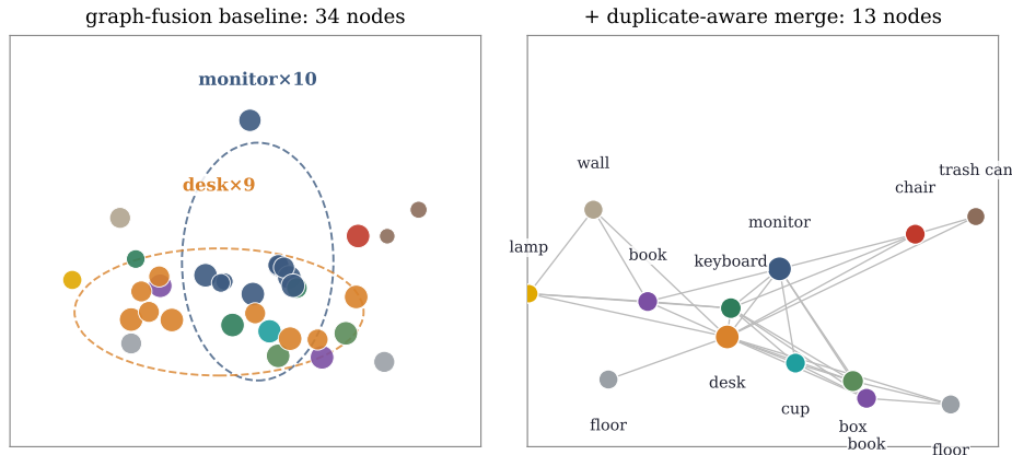
Fig. 1. Duplicate-aware fusion on a real desk scene ( freiburg1_desk , ten views), fused-node centroids projected onto their top two principal axes. Left: cross-view GRAPH-FUSION leaves the single monitor as ten nodes and the desk as nine (dashed rings) — the over-counting that dominates the precision loss. Right: the duplicate-aware merge collapses same-label overlapping nodes into one object each ( 34 \rightarrow 13 nodes), recovering a clean labeled object-relation graph. (Merging is shown by 3D proximity for this illustration; the benchmark metric uses 3D-box IoU, Section 4.3.)
