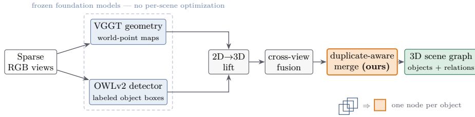
Fig. 2. The pipeline. Sparse RGB views feed two frozen foundation models—VGGT for world-point geometry and OWLv2 for open-vocabulary labeled boxes. Detections are lifted to 3D, fused across views into object nodes, and annotated with spatial relations. Our one addition is a post-fusion duplicate-aware merge (amber): same-label nodes whose 3D boxes overlap are collapsed into a single object, correcting the over-counting that cross-view fusion leaves behind.
