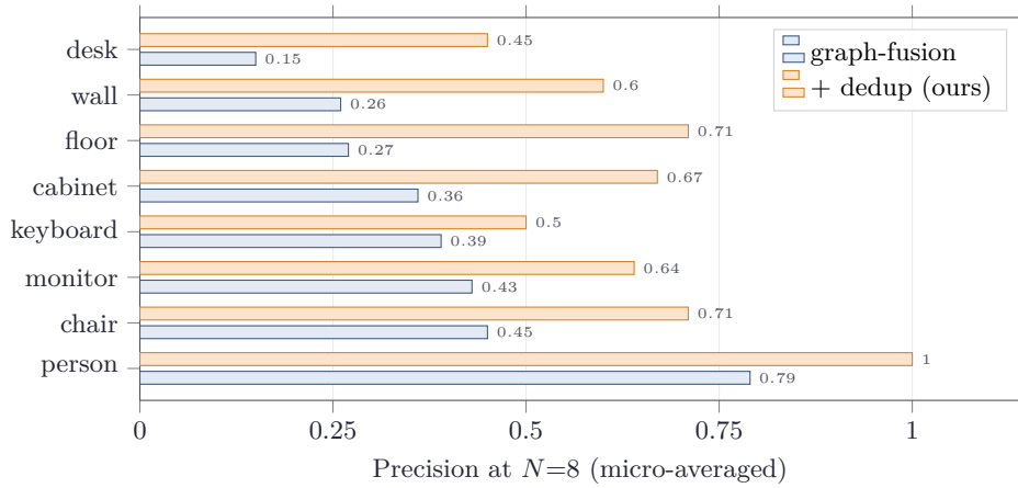
Fig. 5. Where the gain comes from: per-class precision at eight views for the over-counted classes (Table 6). Duplicate-aware fusion sharply recovers precision on the classes the lifted system over-counts ( desk 0.15 \rightarrow 0.45, floor 0.27 \rightarrow 0.71, monitor 0.43 \rightarrow 0.64) while leaving recall unchanged for almost every class. The error it fixes is over-counting of correctly-found objects, not mislabeling.
