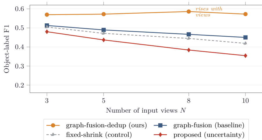
Fig. 4. Object-label F1 vs. number of input views on the independent 28-scene reference. Every prior cross-view fusion variant degrades as views are added—more frames yield more un-collapsed duplicate detections, costing precision. Duplicate-aware fusion (ours, amber) is the only variant whose accuracy rises toward the dense end and is best at every view count, while the uncertainty-aware gate (brick) sits below even the uninformed control. Values match Table 2.
