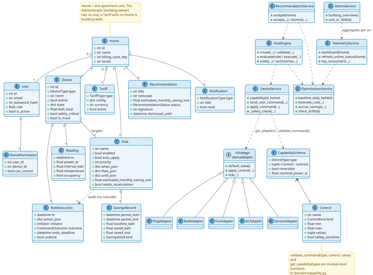
Figure 5.5. Class diagram. The unit (a Home occupied by one Resident) is the aggregate root; the device-adapter interface hierarchy and the capability-schema value objects drive device behaviour and command validation. The user-device control grant is reified by an explicit permission class, and the rule-to-execution dependency is deliberately non-cascading so that deleting a rule preserves its audit trail.
