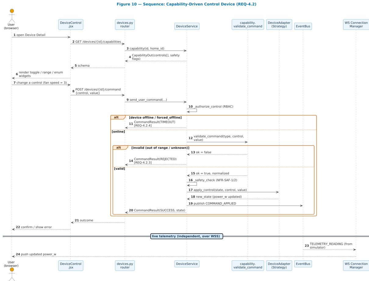
Figure 5.6. Sequence: capability-driven device control. The command is validated against the same capability schema used to render the control, then applied through the device-adapter interface, and the new state is broadcast over the event bus to all connected front-ends.
