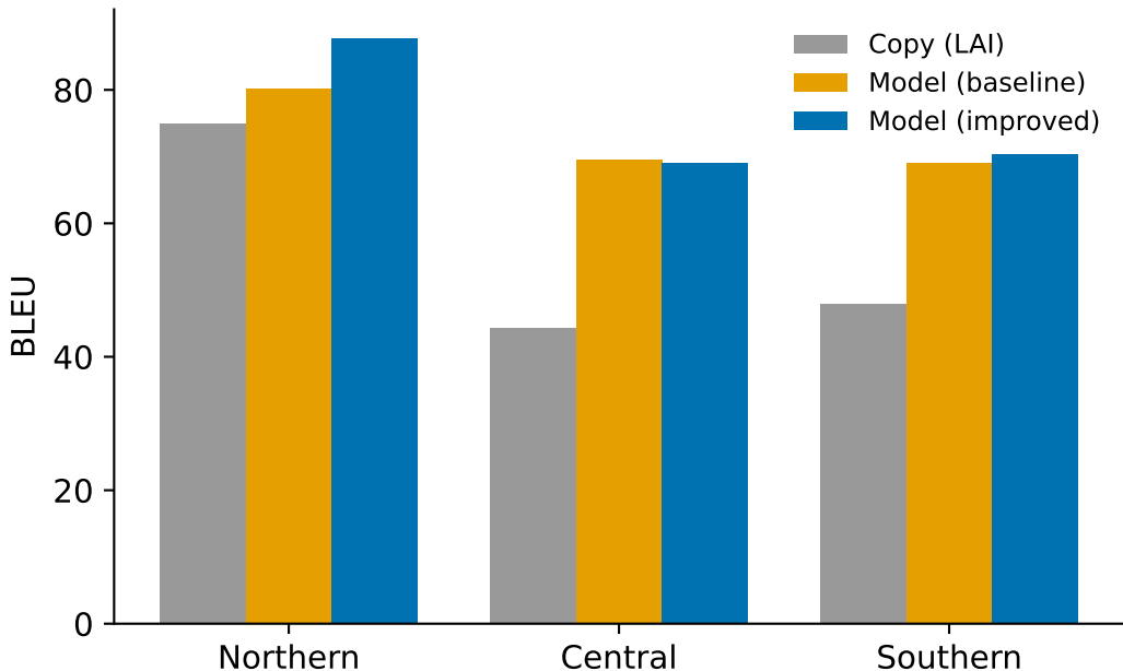
Standard→Dialect: copy baseline vs model
