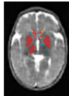
Annotation disagreement
