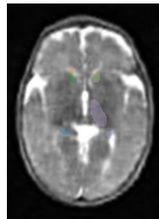
LF-edited mask
