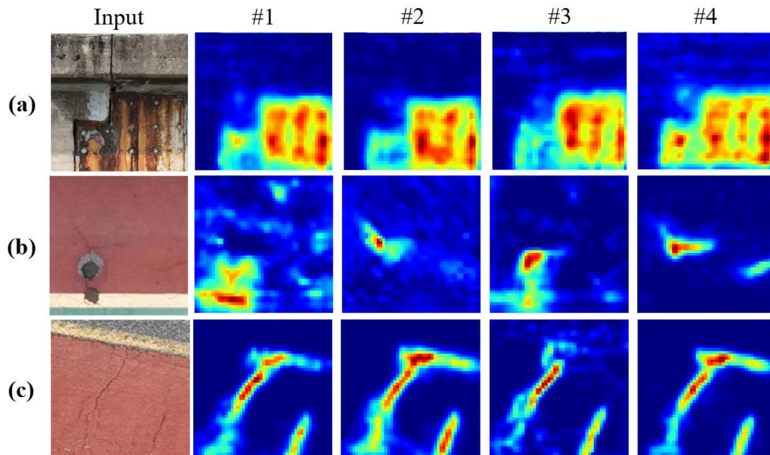
Figure 8: Visualization of prototype-activated feature maps at feature map F2. The first column presents the input images, while columns #1 to #4 display the corresponding feature maps.
