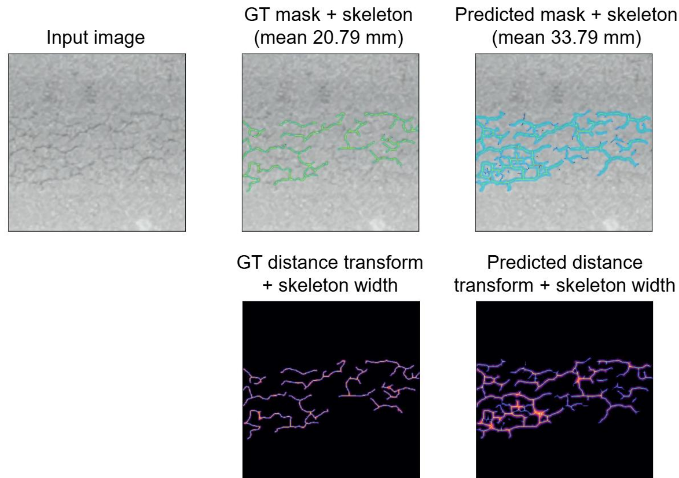
Figure 12: Discrepancies in width measurement arise due to differences in topological completeness. Although standard error metrics heavily penalize the model for overprediction, visual assessment indicates that the model identifies a more structurally realistic and interconnected fracture network, which is absent from the baseline manual labels. Note: Skeletonization reduces the segmented mask to a 1-pixel-wide centerline to represent the structural topology, and the distance transform calculates the local crack width by measuring the shortest Euclidean distance from this centerline to the nearest defect boundary.
