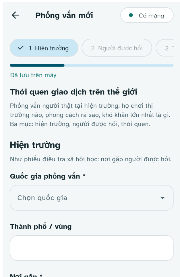
Figure 2. Form step 1 (site): country dropdown and required place field.
