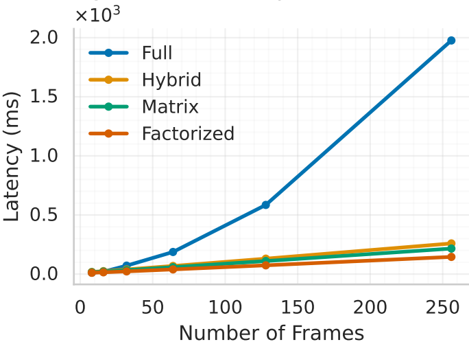
Average Forward Latency vs Number of Frames
