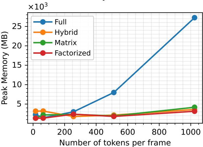
Peak GPU Memory vs Number of Tokens
