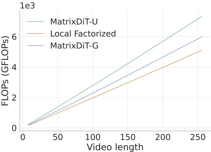
FLOPs vs Number of Frames (forward)
