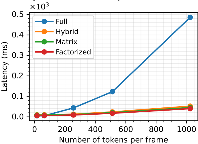
Average Forward Latency vs Number of Tokens
