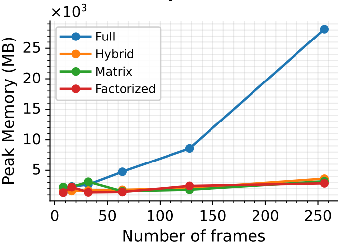
Peak GPU Memory vs Number of Frames
