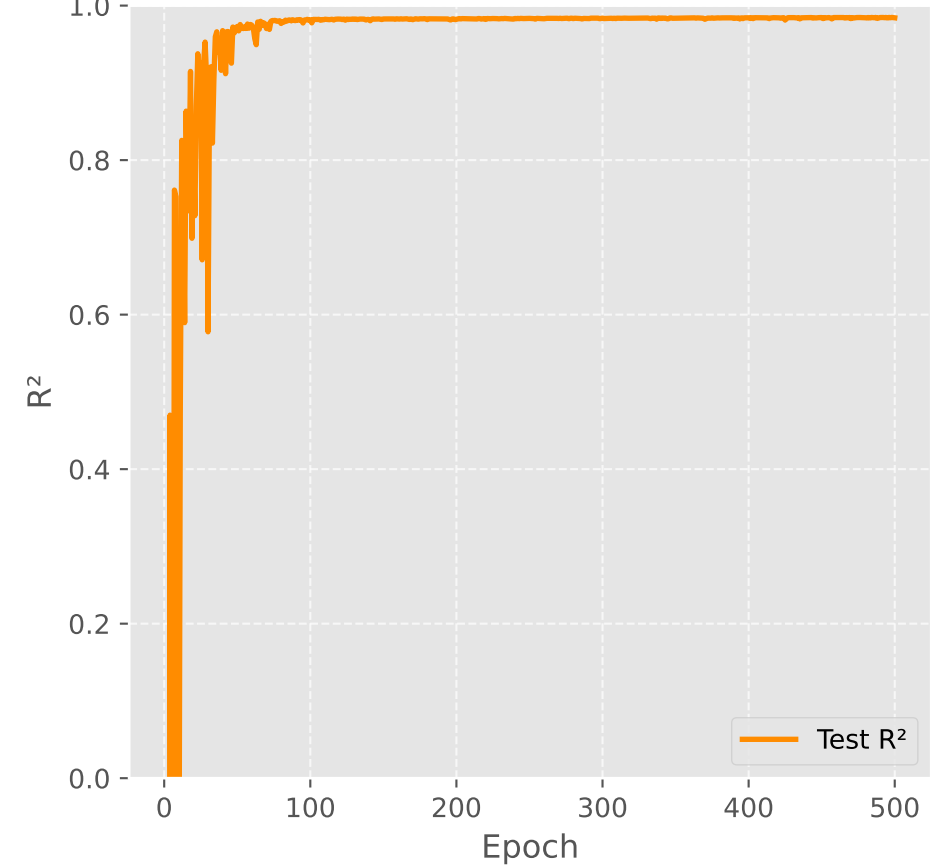
R 2
