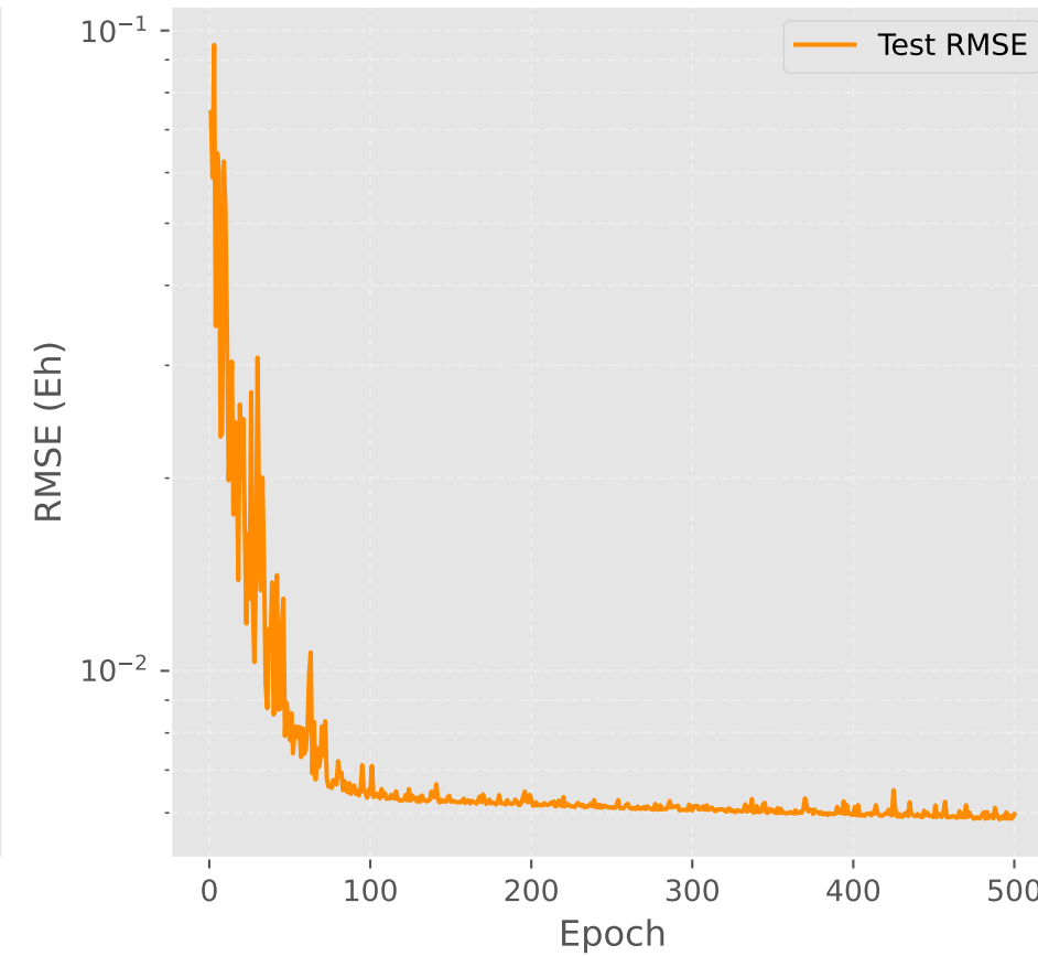
RMSE
