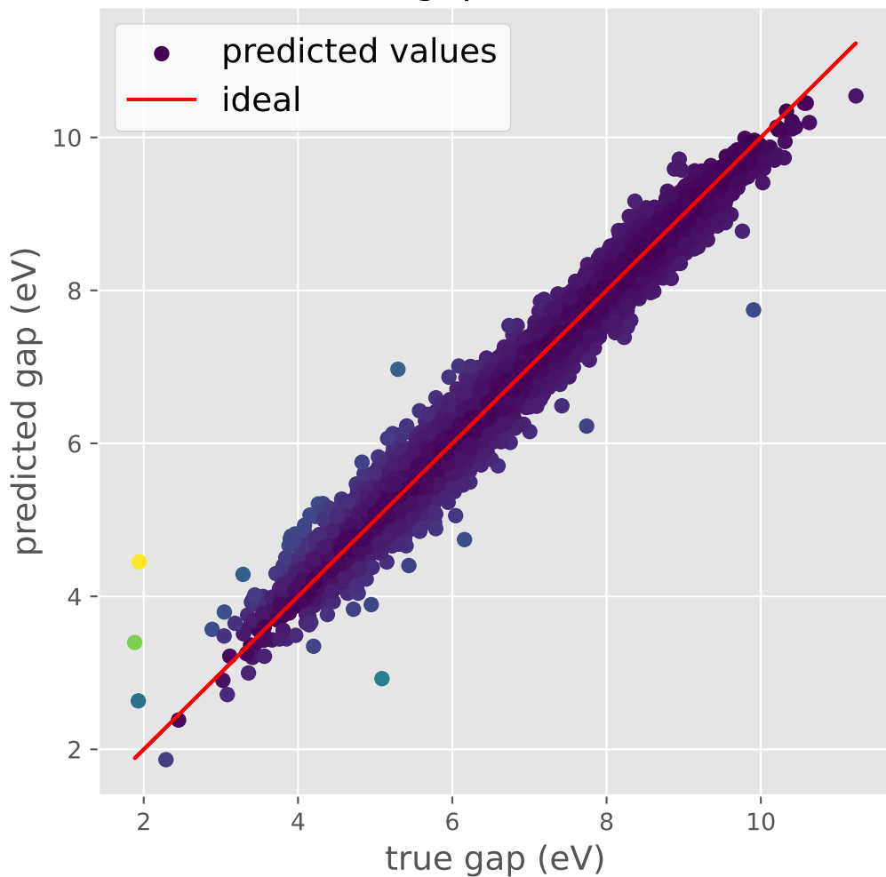
SchNet prediction plot gap (eV)
