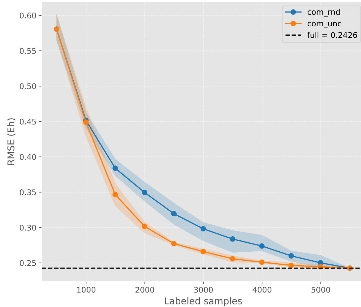
RMSE (Eh)
