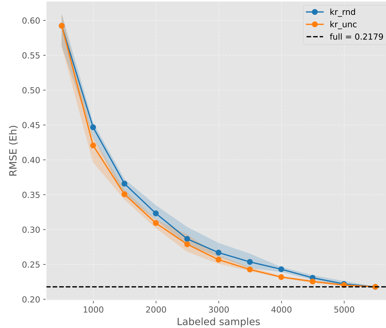
RMSE (Eh)
