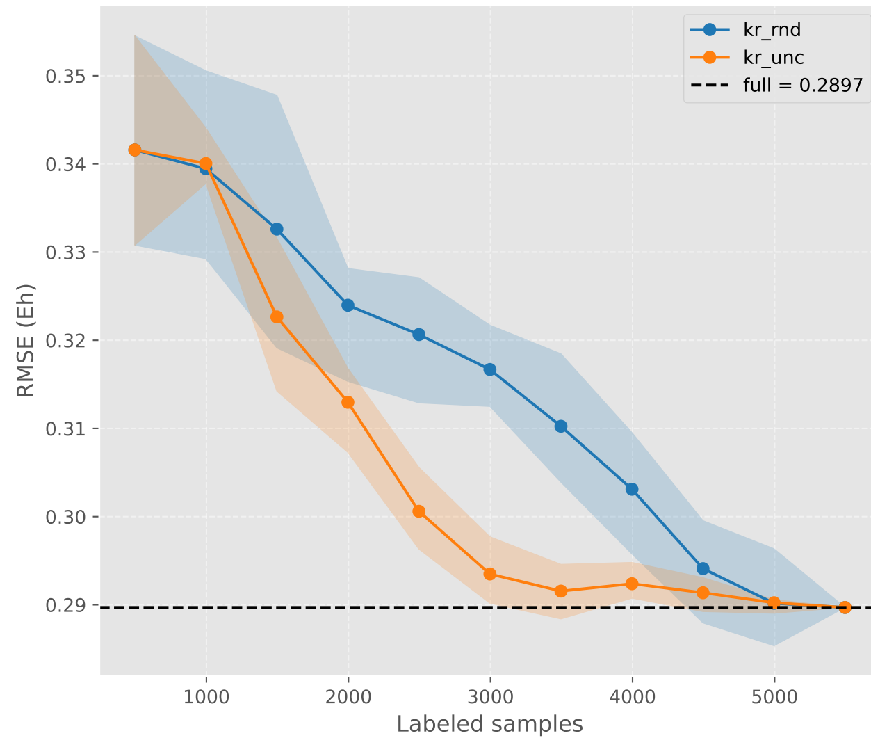
RMSE (Eh)
