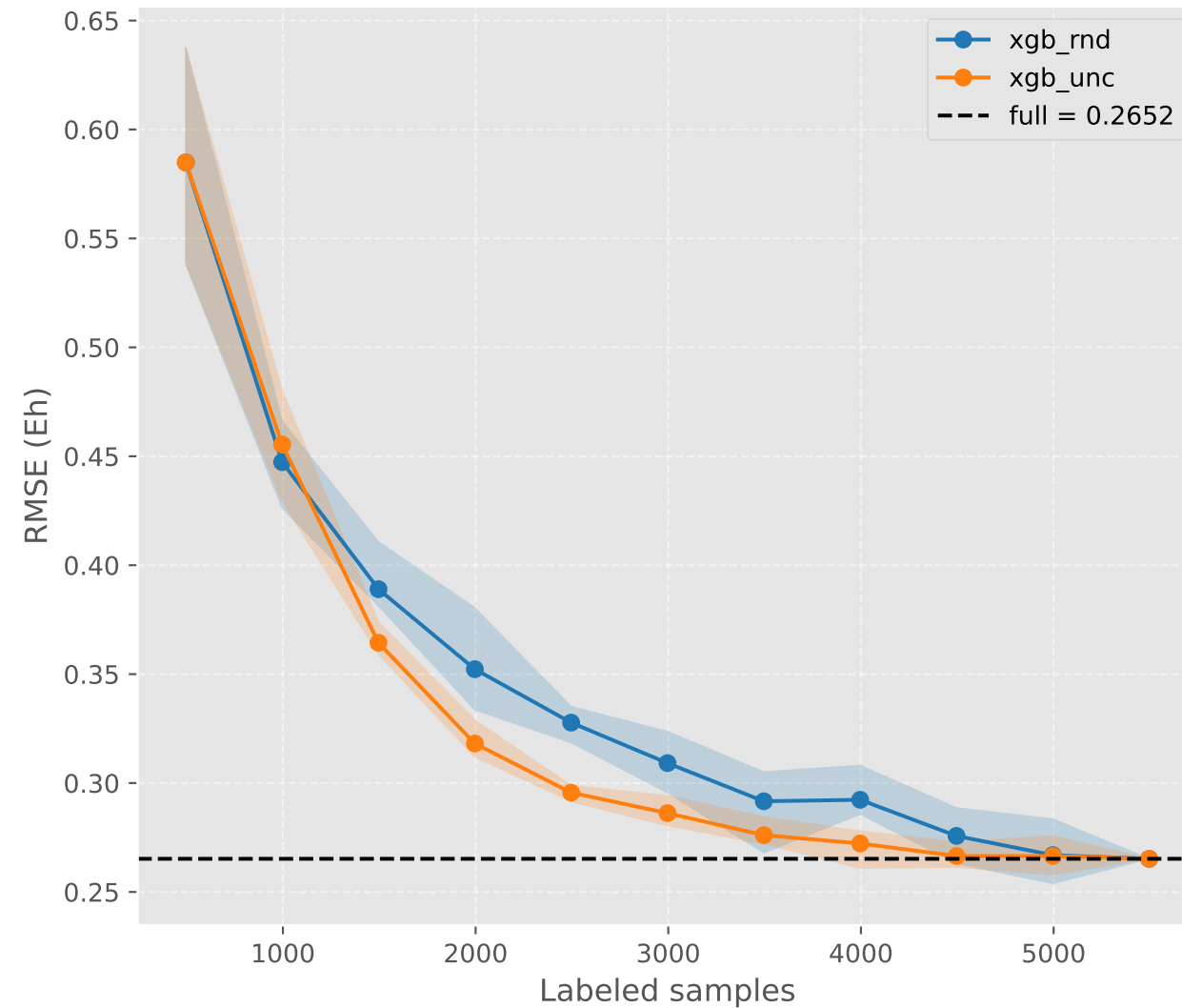
RMSE (Eh)
