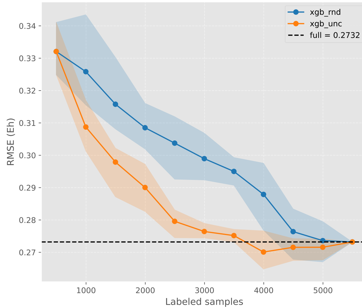
RMSE (Eh)
