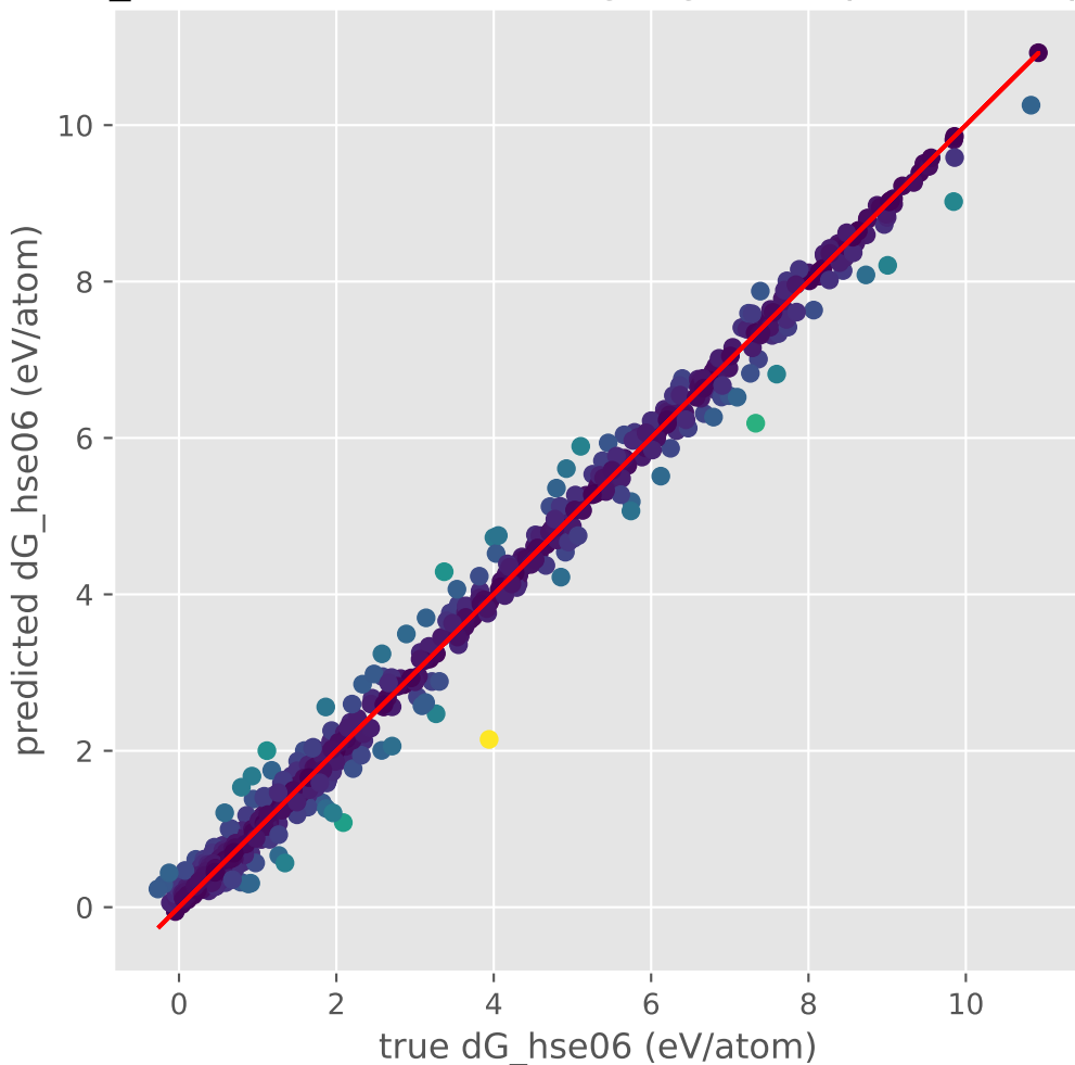
dG_hse06 (eV/atom) VotingRegressor prediction plot
