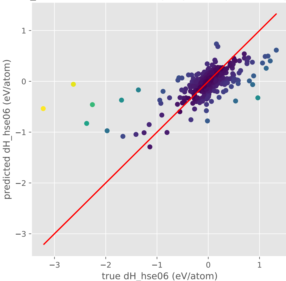
dH_hse06 (eV/atom) VotingRegressor prediction plot
