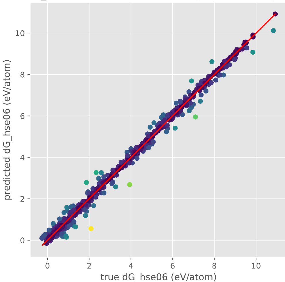
dG_hse06 (eV/atom) KernelRidge prediction plot
