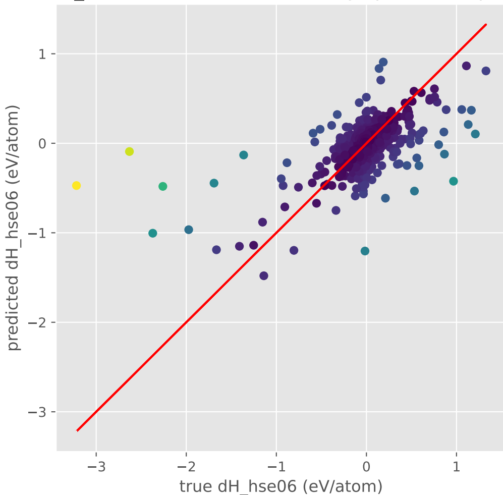
dH_hse06 (eV/atom) KernelRidge prediction plot
