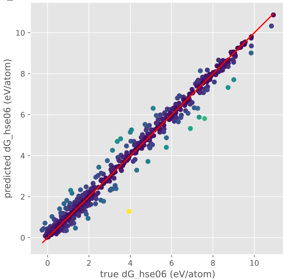
dG_hse06 (eV/atom) RandomForestRegressor prediction plot
