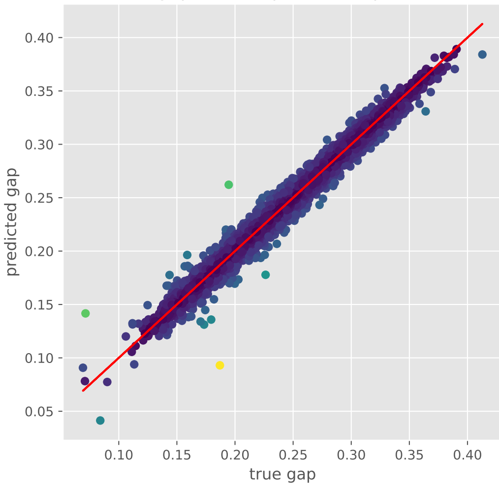
gap SchNet prediction plot
