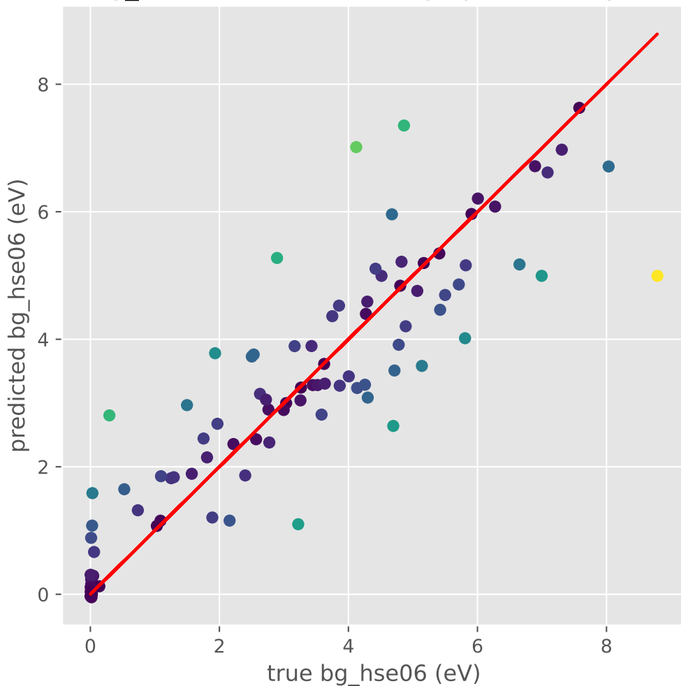
bg_hse06 (eV) KernelRidge prediction plot
