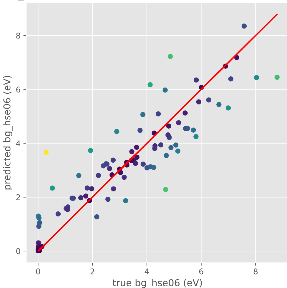
bg_hse06 (eV) RandomForestRegressor prediction plot
