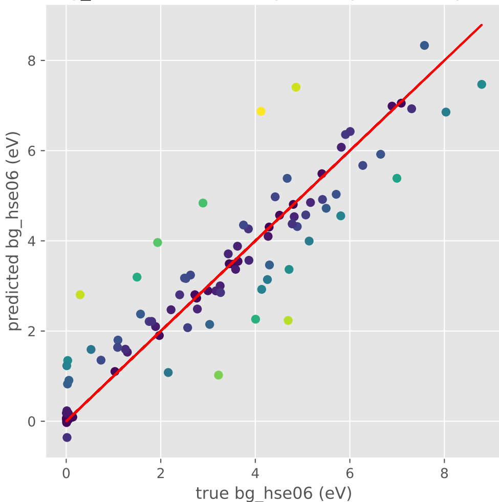
bg_hse06 (eV) XGBRegressor prediction plot
