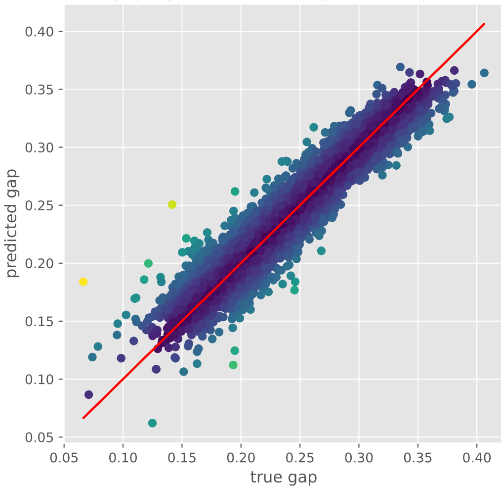
gap Nystroem+Ridge prediction plot
