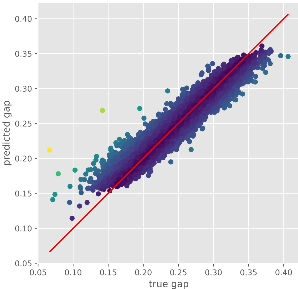
gap RandomForestRegressor prediction plot
