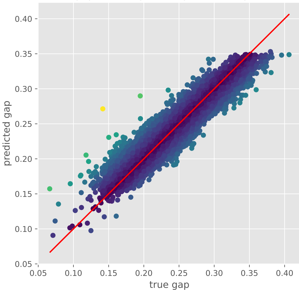
gap XGBRegressor prediction plot
